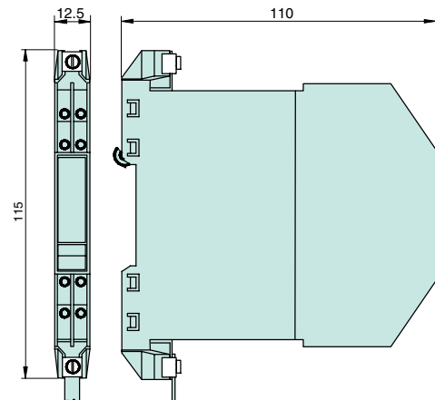
Figure 1.11 Mechanical features
