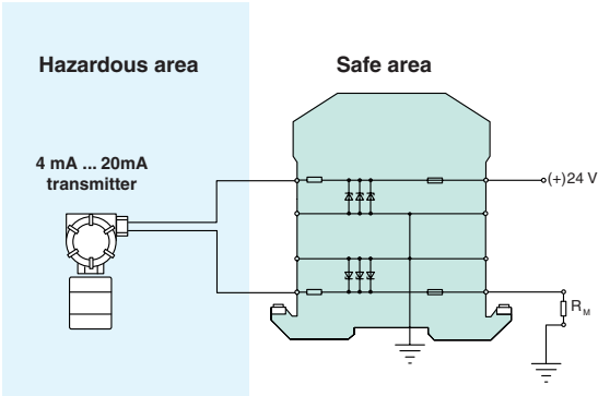
Figure 1.5 Two-channel Zener barrier
