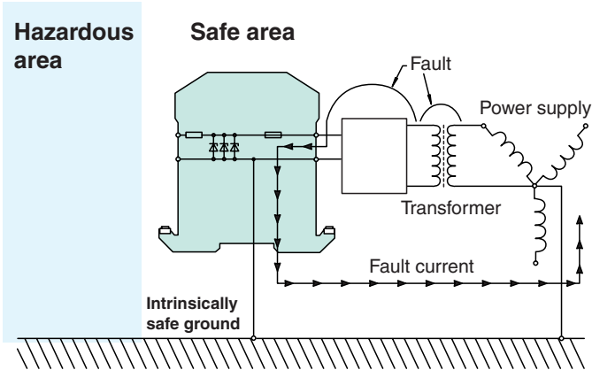
Figure 1.7 Grounded Zener barriers The system must have its own independent ground conductor, through which no supply system current flows.
