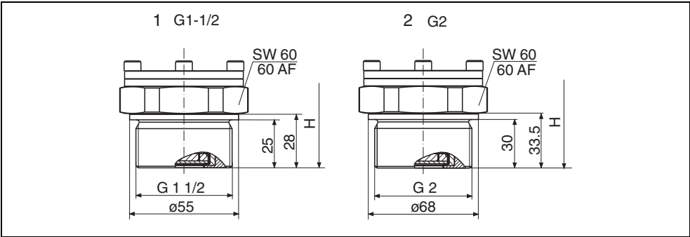
Process connections PPC-M51, thread ISO
