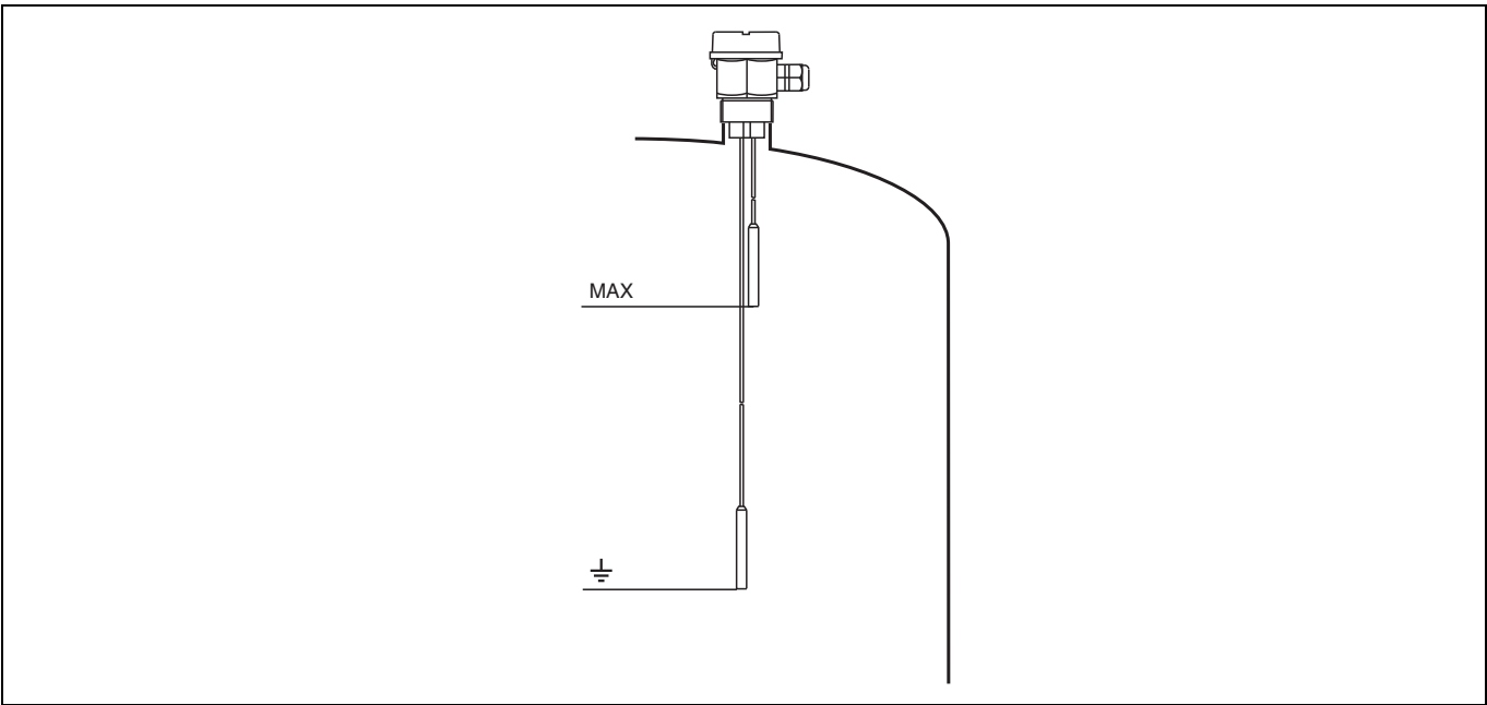
Level limit detection (MAX) MAX and MIN detection for compact instrumentation version only possible with \Delta s .
