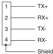
Ethernet
